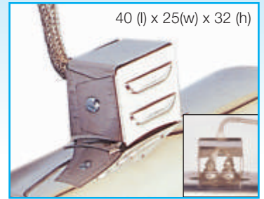
SS 304 Terminal Box with Screw Post Terminals and 10" Long Cable
